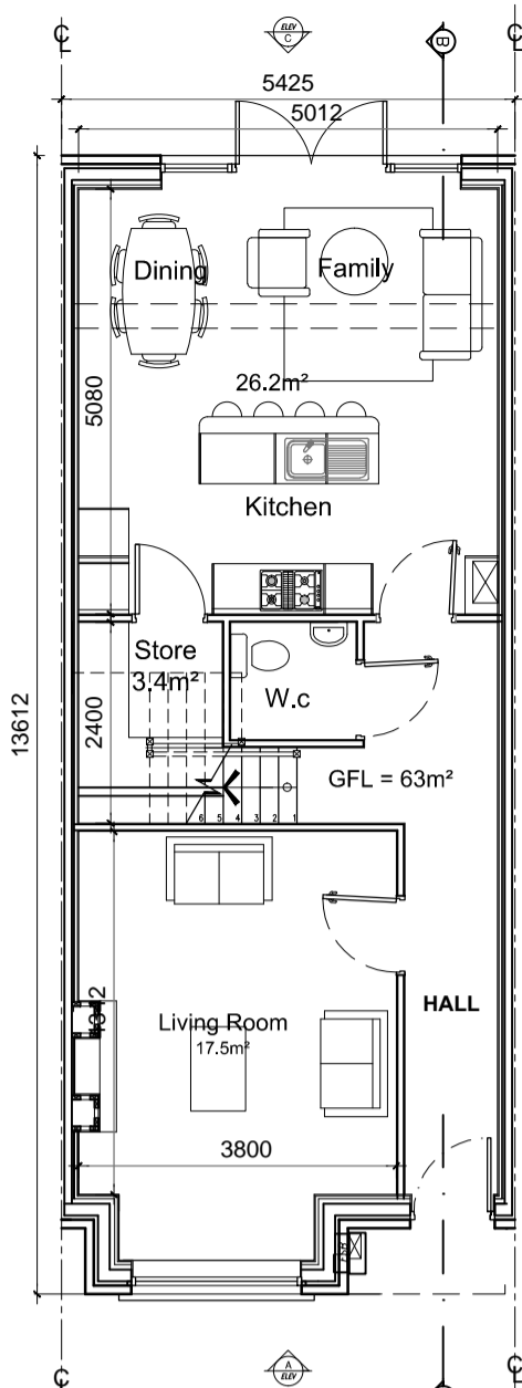
Ground Floor Plan Right Entry area 63m 2 / 678 ft 2 O/ALL AREA 114.4m 2 / 1,231 ft 2
