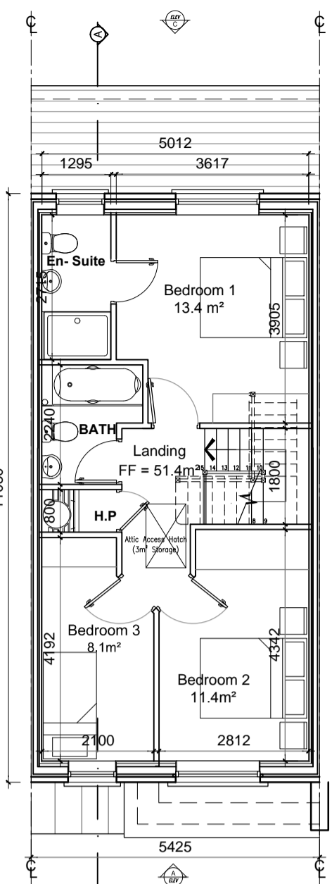
First Floor Plan Left Entry area 51.4m 2 / 553 ft 2
