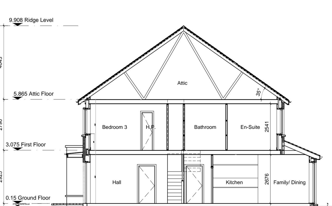
SECTION B-B
