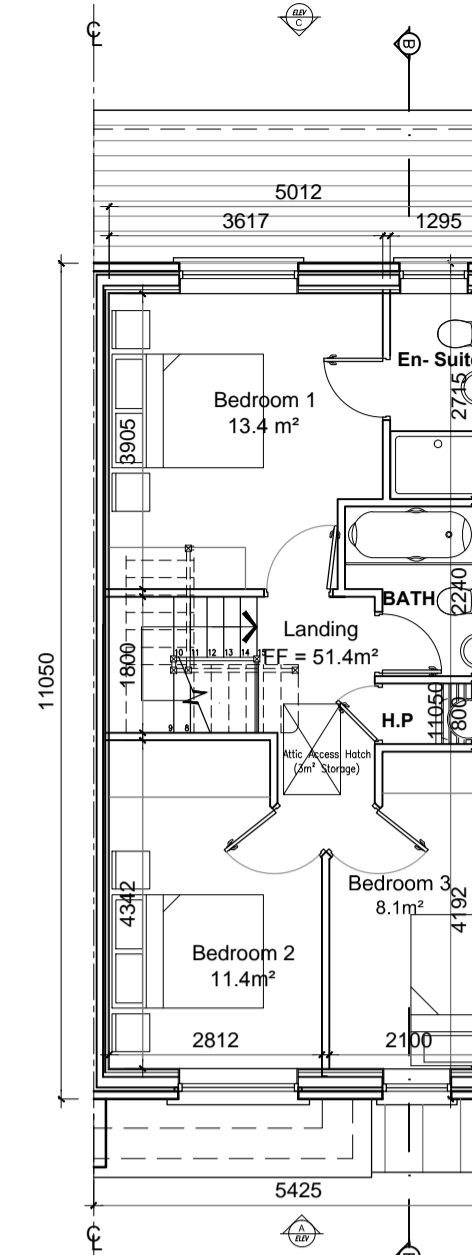
First Floor Plan Right Entry area 51.4m 2 / 553 ft 2
